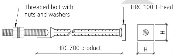
Fig. 3 HRC 720 with bolt, nuts and washers, and combined with T-heads from the HRC 100 series (shown here with HRC 120)
